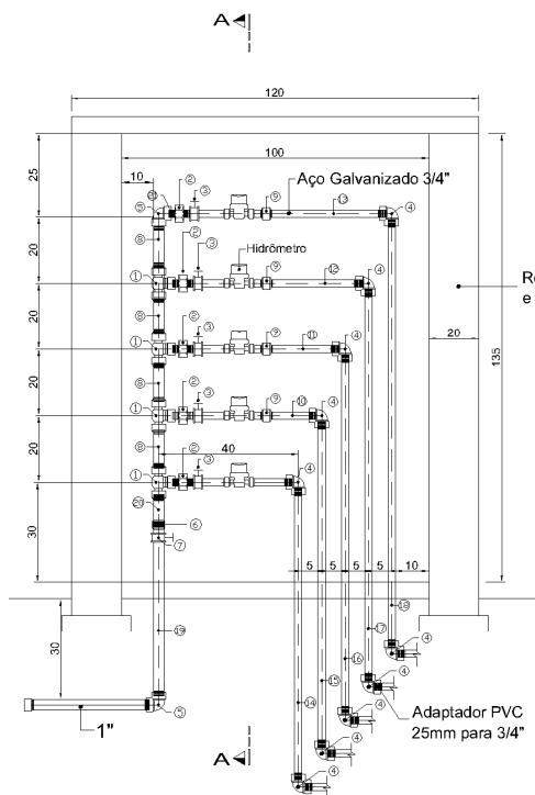
VISTA FRONTAL
